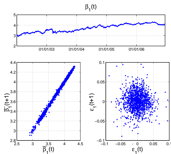
Figure 1. Removal of temporal structure. (Top) Shows the data curve fitting coefficient \beta_1(t) ; (Bottom left) Scatter plot of \tilde{\beta}_1(t) = \beta_1(t) - \hat{\mathbf{m}} - \hat{\mathbf{d}}t and its lag revealing its AR nature; (Bottom right) The residuals \tilde{\epsilon}_1(t) scatter plot – after the AR structure is removed from \beta_1(t) .
